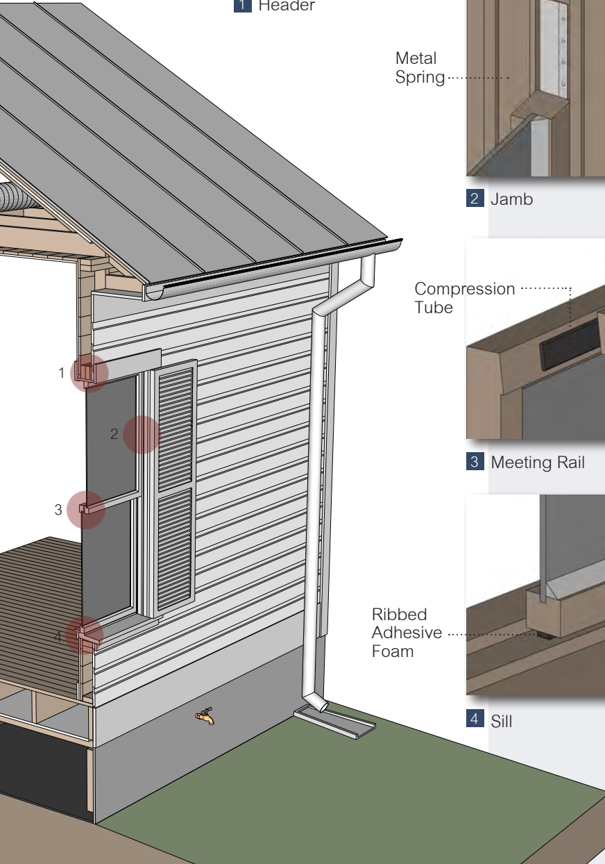
1 Header
